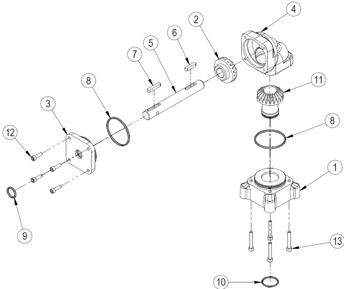
EXPLODED VIEW FOR IW100 GEARBOX OPERATIONS
