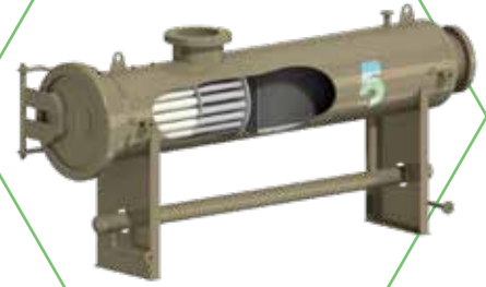
FILTER SEPARATORS
