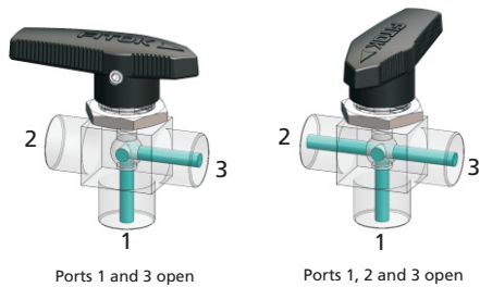
Ports 1 and 3 open
